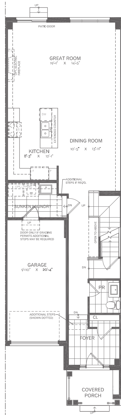
Ground Floor - Elevation C
