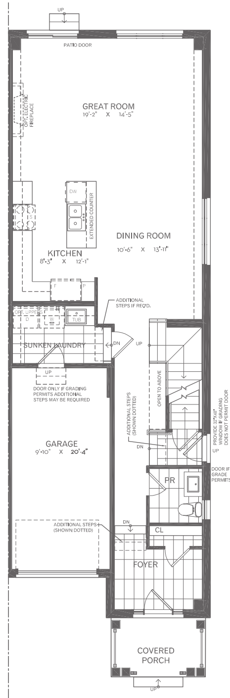
Ground Floor - Elevation D
