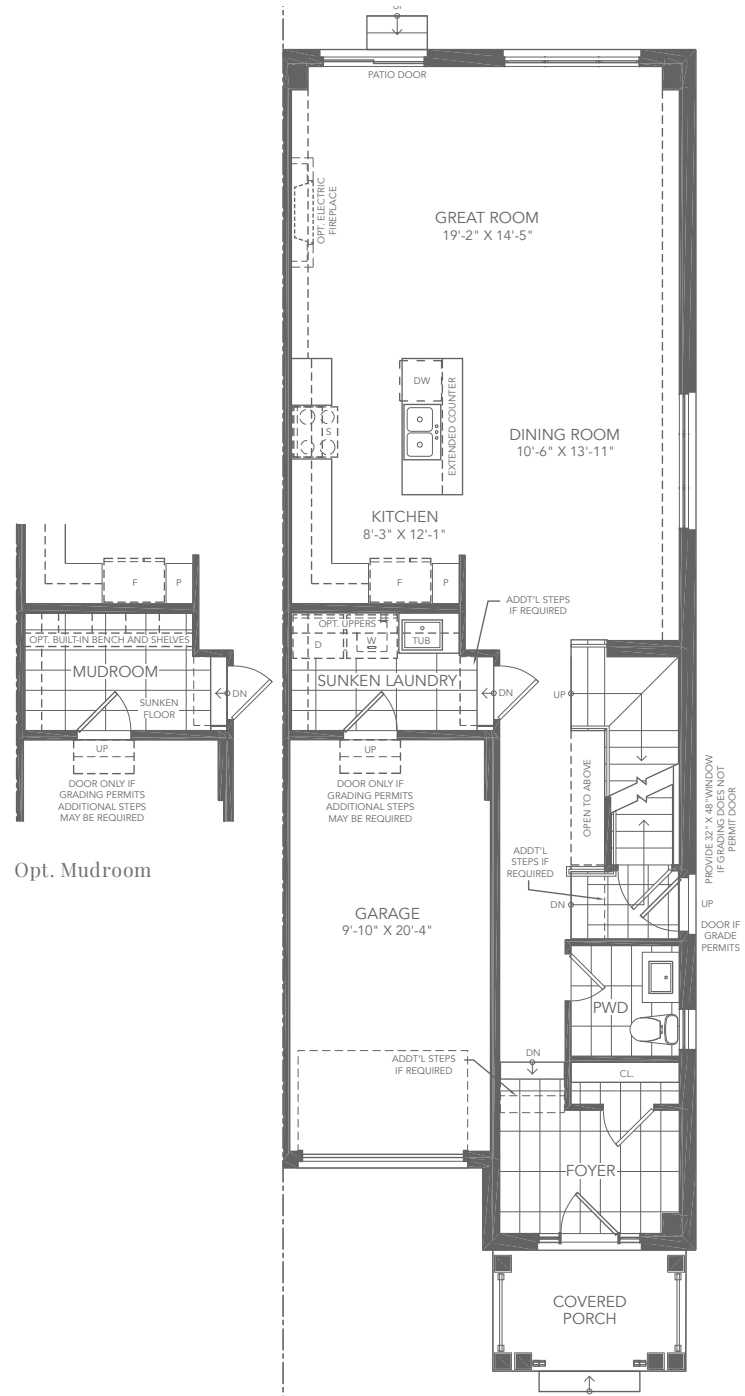
Ground Floor - Elevation J
