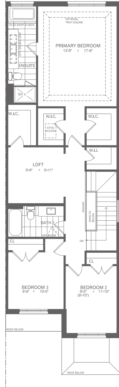
Second Floor - Elevation D
