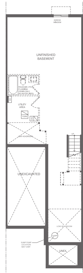
Basement - Elevation A
