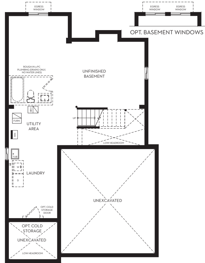
BASEMENT PLAN
