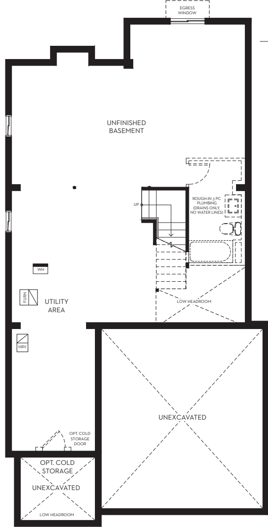
BASEMENT PLAN
