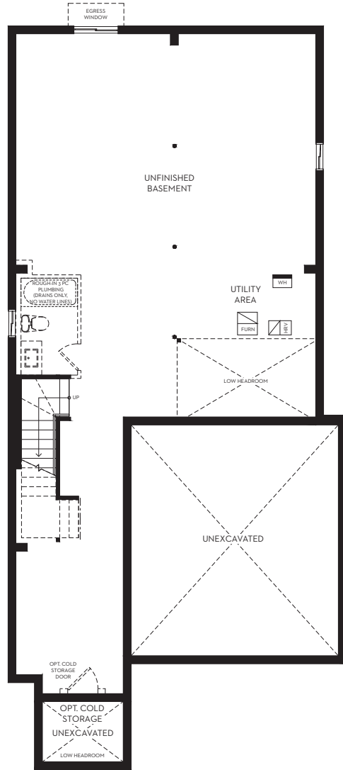
BASEMENT PLAN
