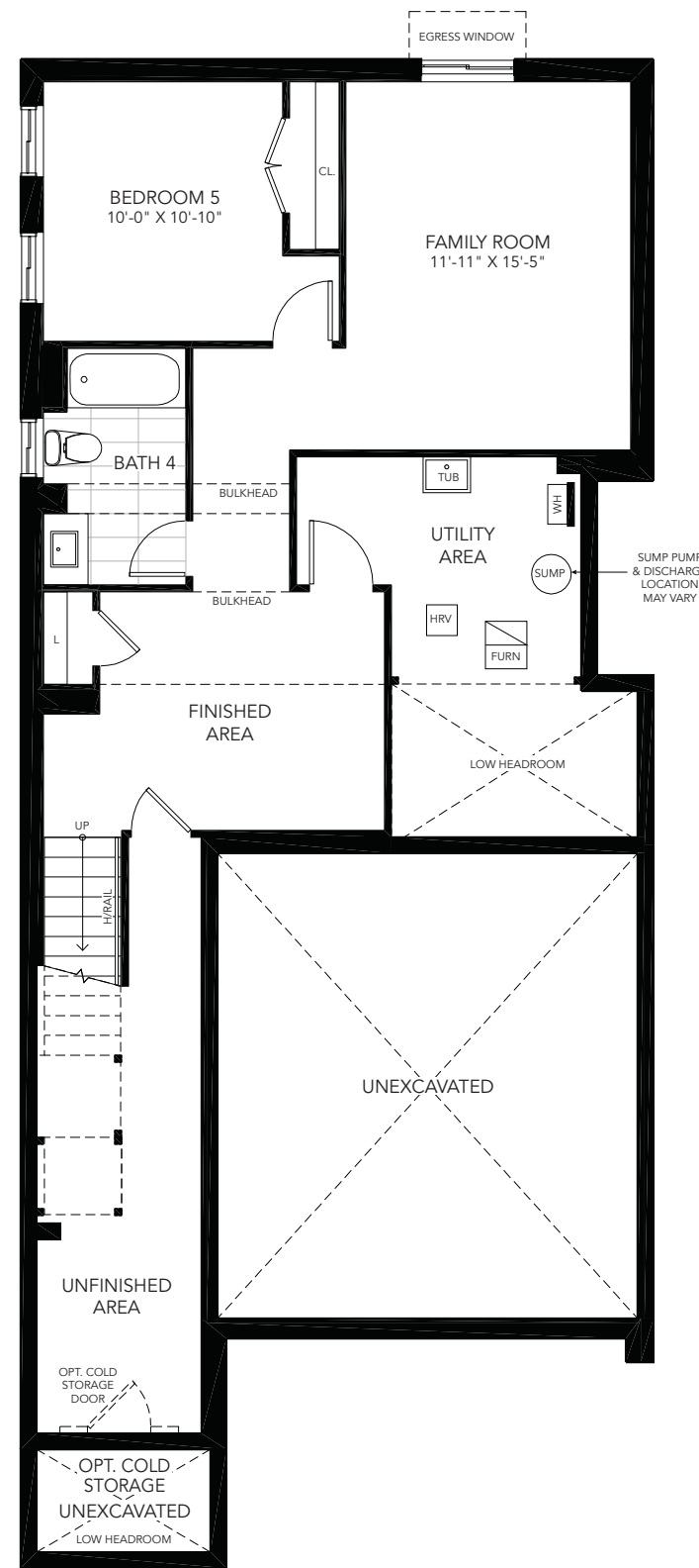
FINISHED BASEMENT PLAN
