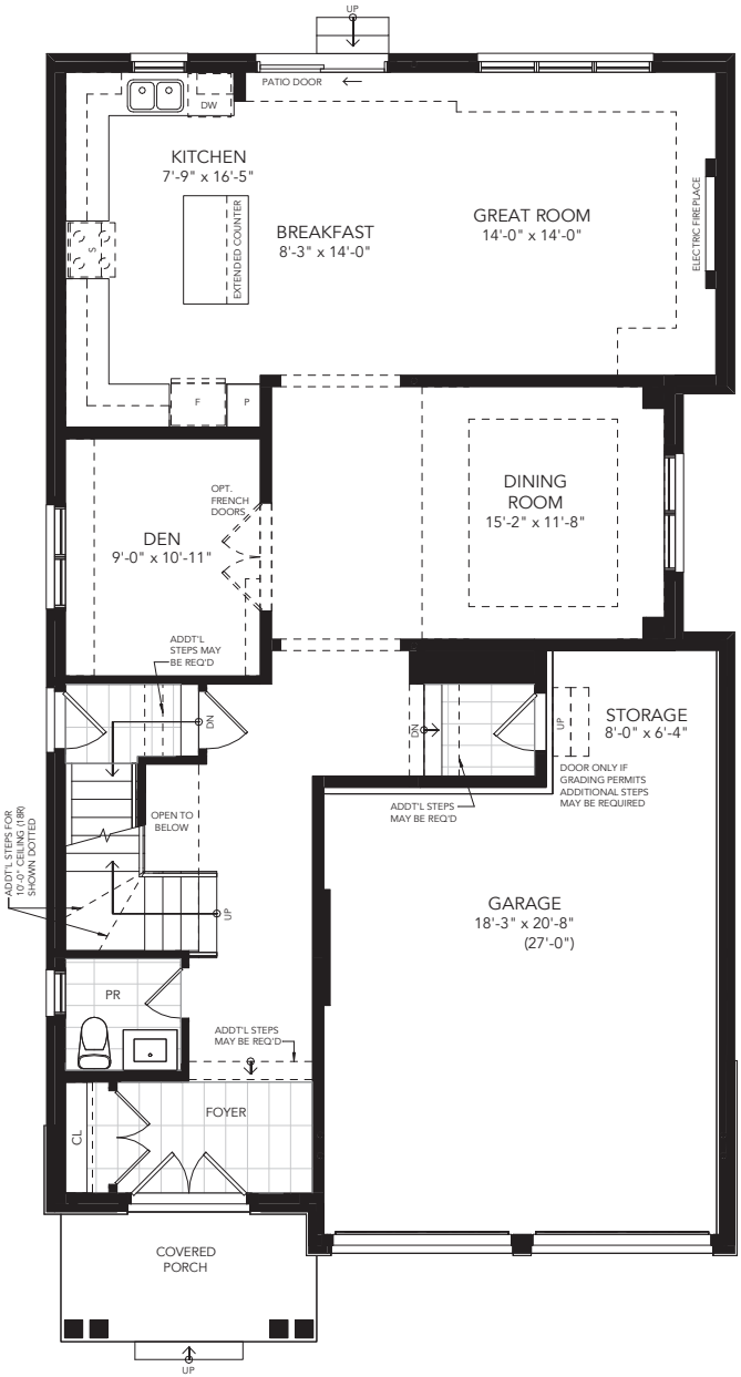
GROUND FLOOR A
