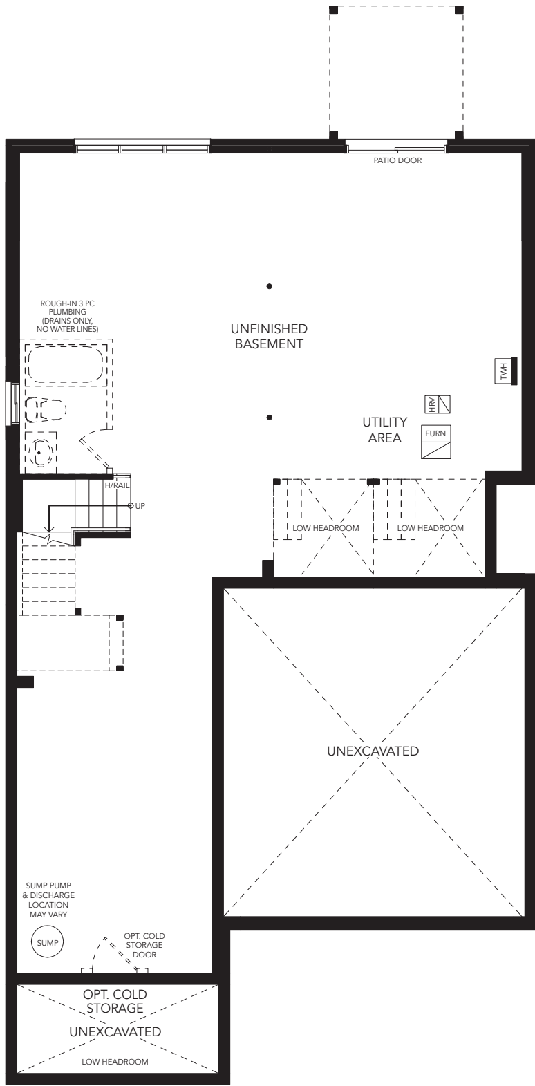
BASEMENT PLAN
