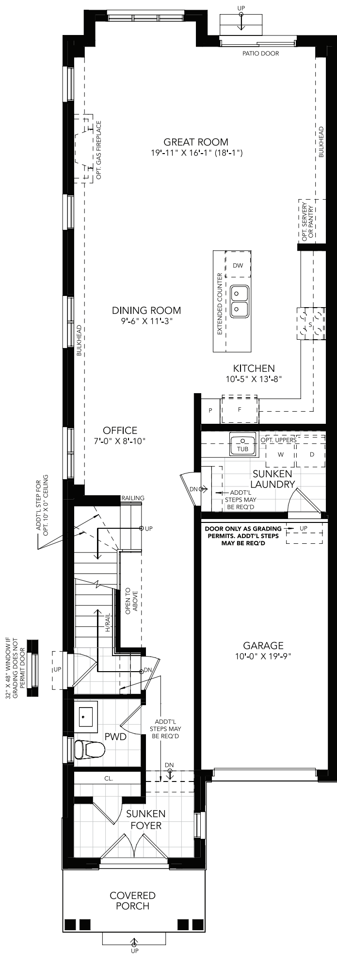
GROUND FLOOR PLAN ELEV. A
