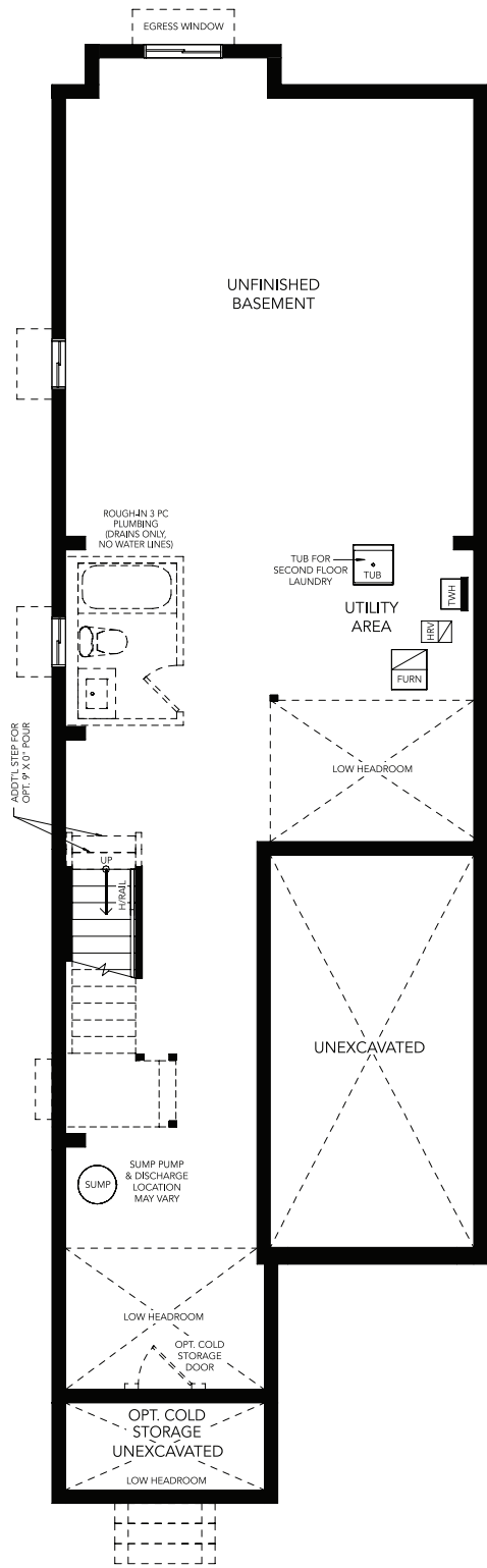
BASEMENT PLAN ELEV. A
