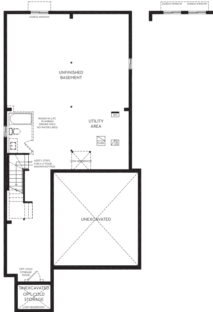
BASEMENT PLAN
