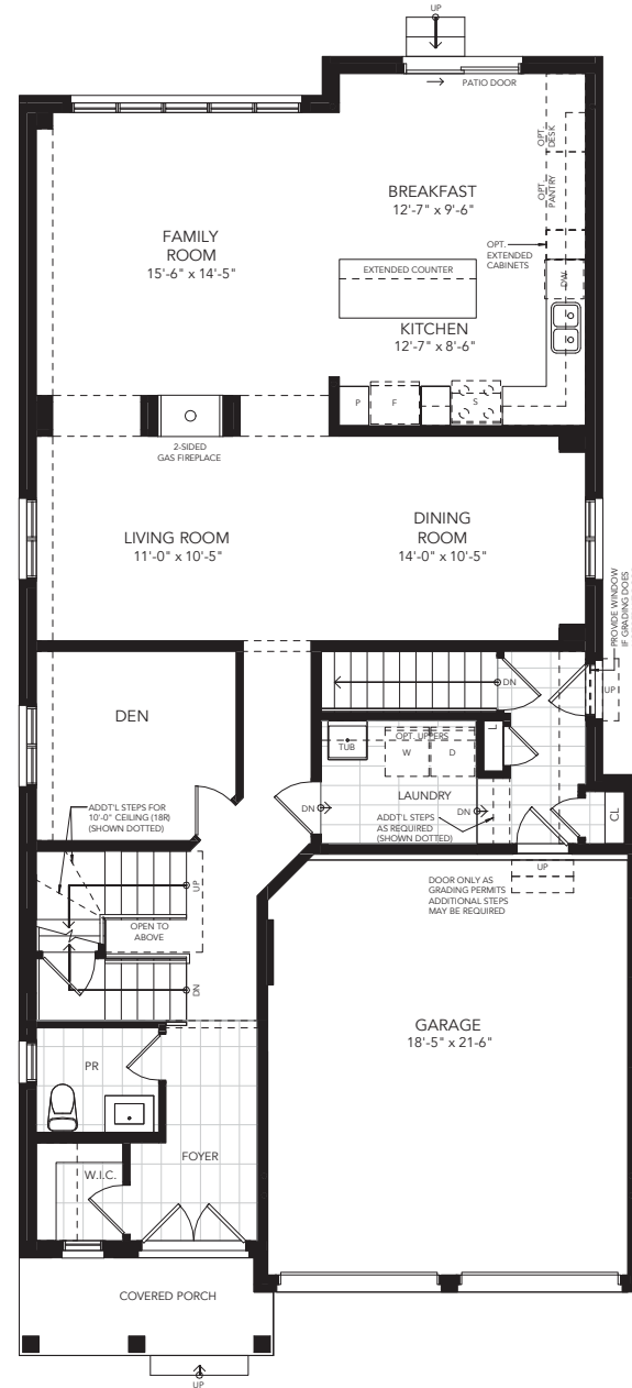
GROUND FLOOR A
