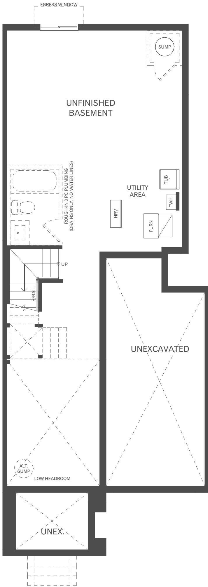
BASEMENT PLAN M
