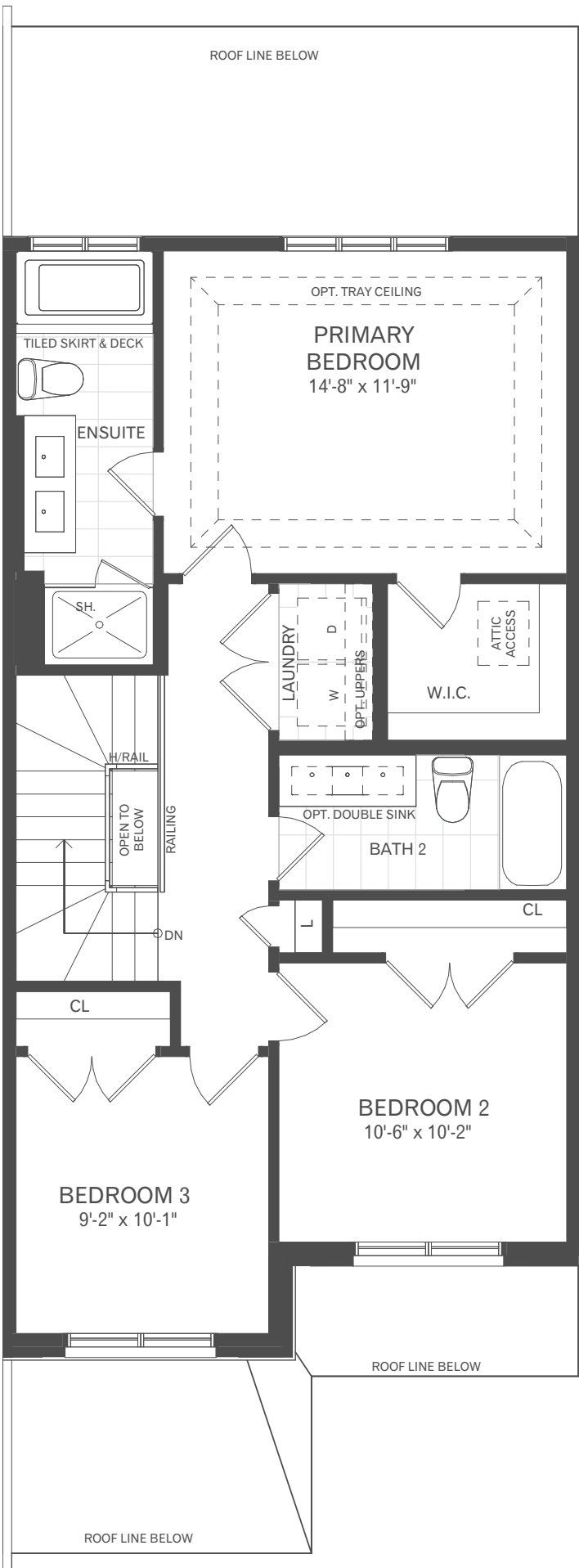
SECOND FLOOR PLAN M
