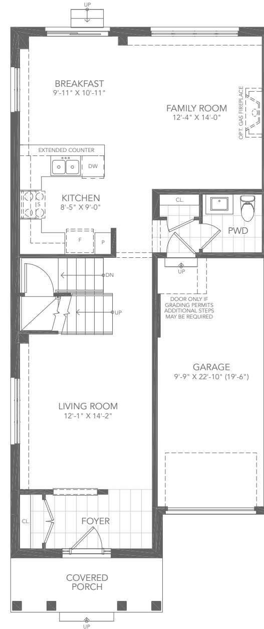
GROUND FLOOR PLAN A
