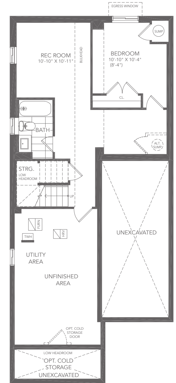
BASEMENT PLAN A
