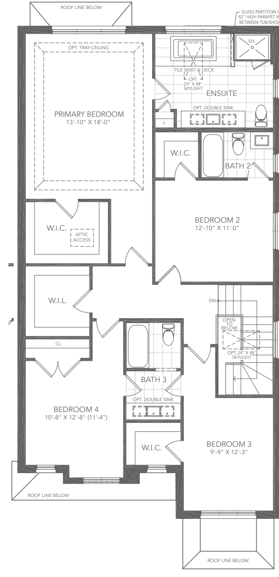
SECOND FLOOR PLAN A
