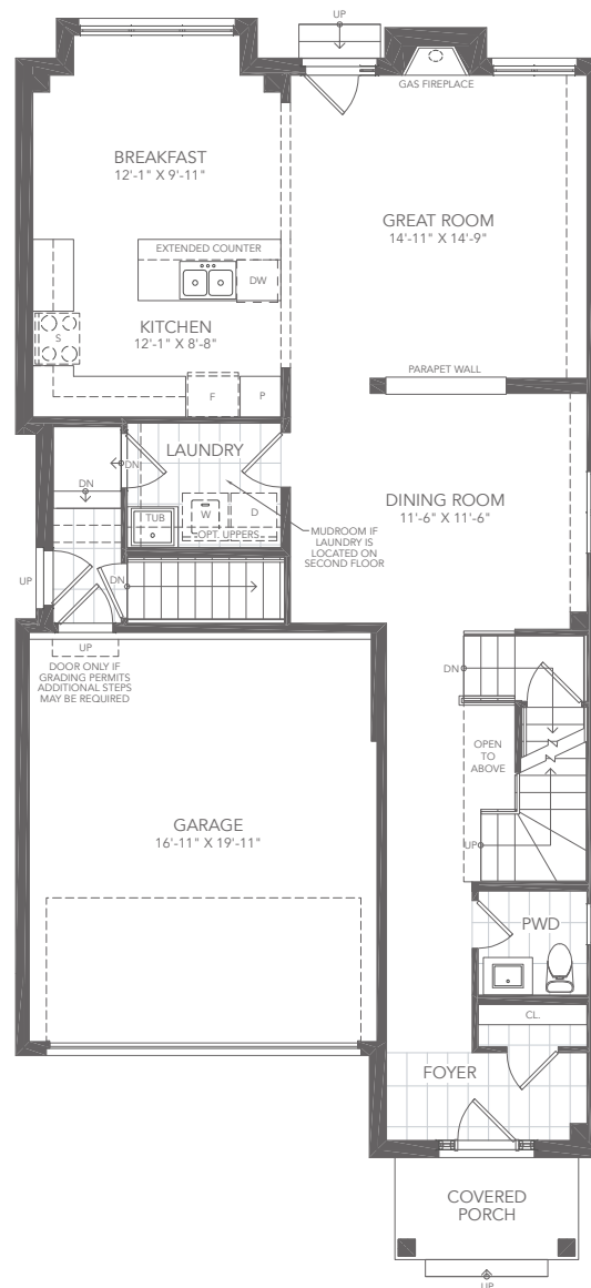
GROUND FLOOR PLAN A
