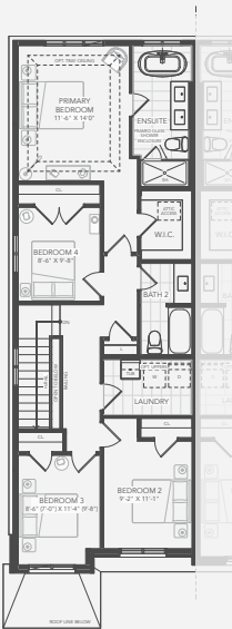
OPTIONAL 4TH BEDROOM SECOND FLOOR PLAN
