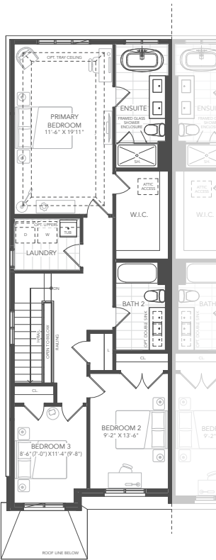
SECOND FLOOR PLAN A
