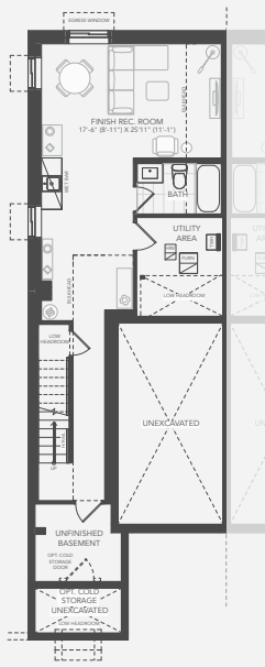
OPTIONAL FINISHED BASEMENT PLAN + 530 Sq. Ft.
