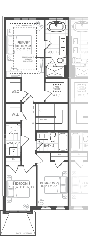
SECOND FLOOR PLAN A
