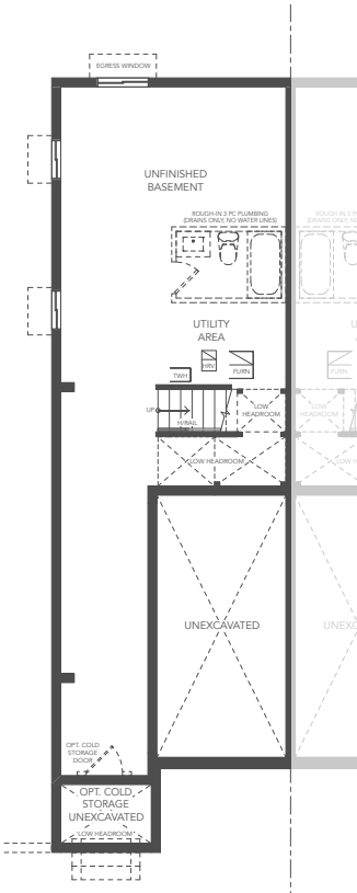
BASEMENT PLAN A
