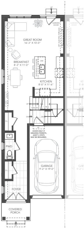
GROUND FLOOR PLAN A
