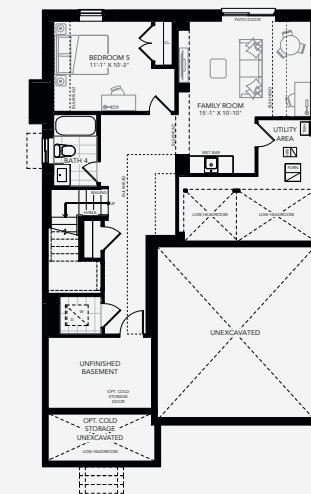
OPTIONAL FINISHED BASEMENT PLAN WALKOUT + 755 Sq. Ft.
