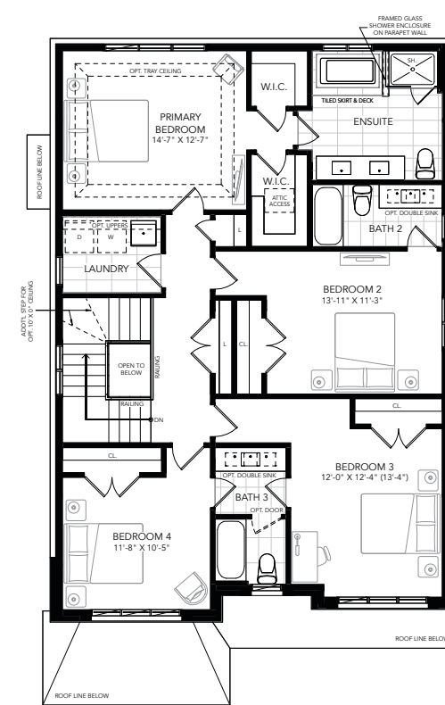
SECOND FLOOR PLAN A
