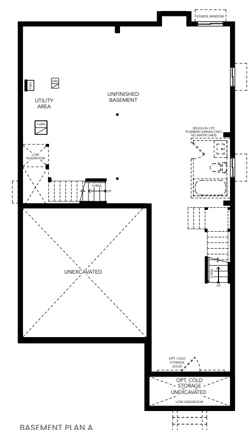
BASEMENT PLAN A
