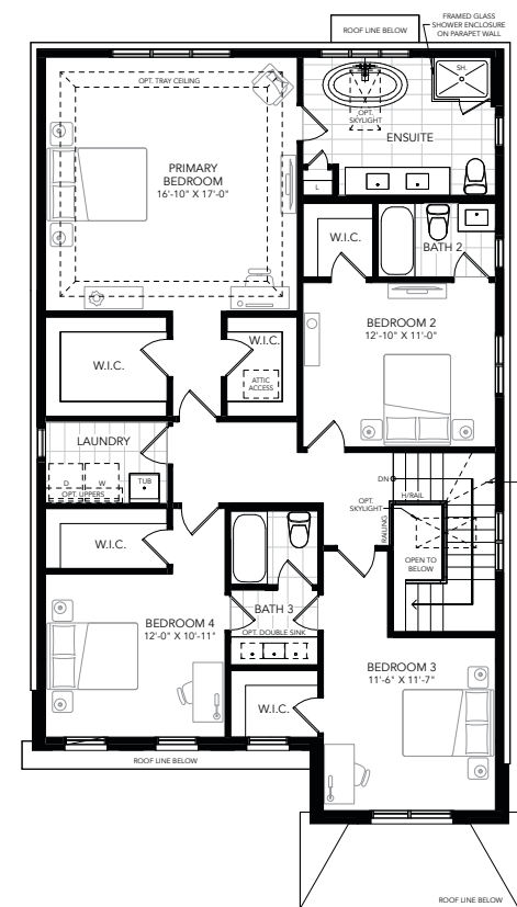
SECOND FLOOR PLAN A
