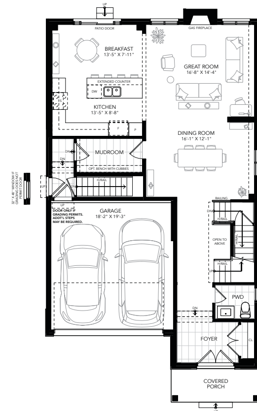
GROUND FLOOR PLAN A
