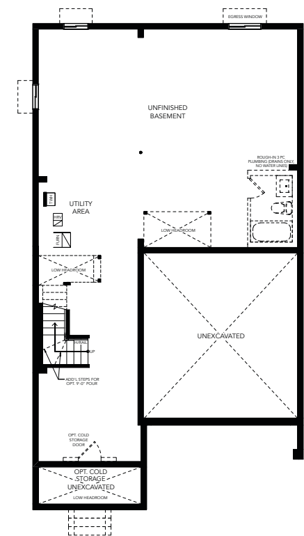
BASEMENT PLAN A
