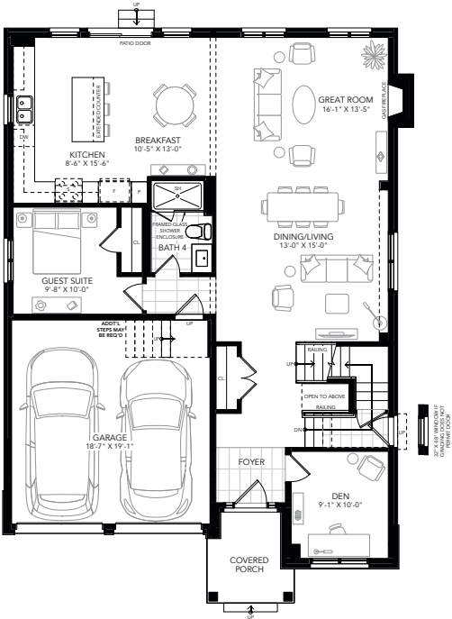
GROUND FLOOR PLAN A
