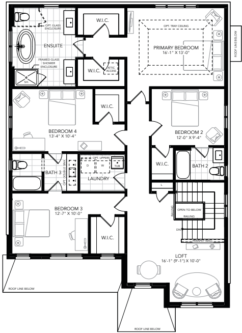
SECOND FLOOR PLAN A
