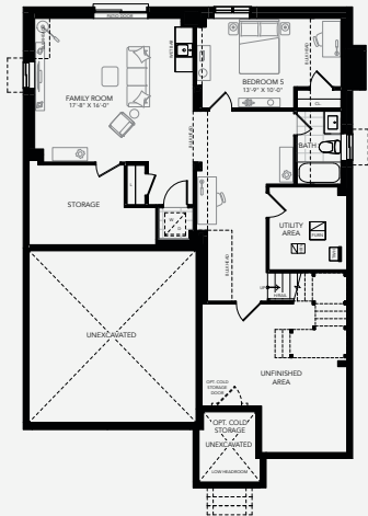
OPTIONAL FINISHED BASEMENT PLAN WALKOUT + 880 Sq. Ft.
