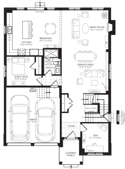
GROUND FLOOR PLAN A
