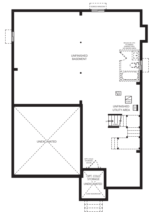
BASEMENT PLAN A
