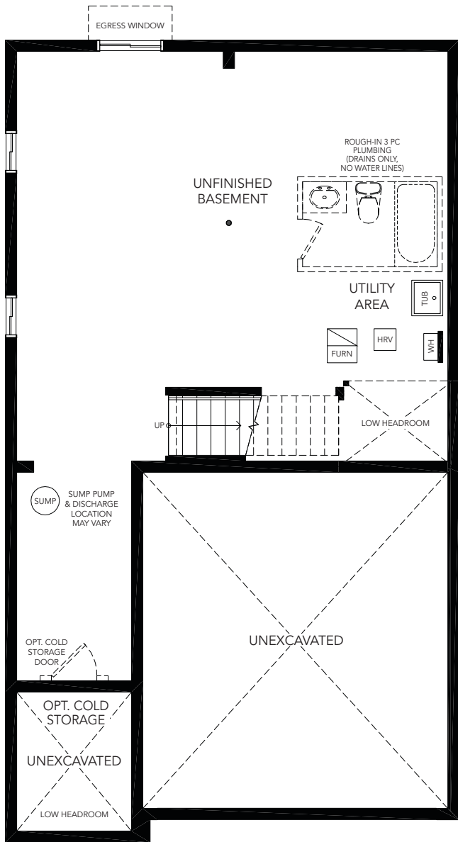
BASEMENT PLAN
