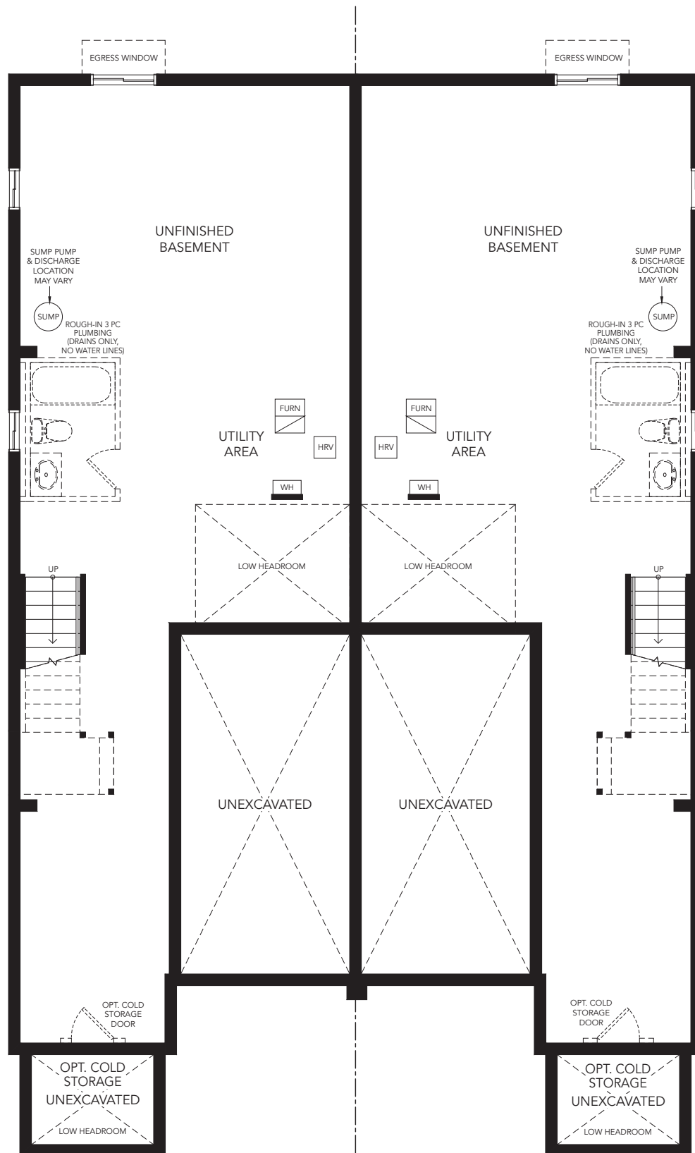
BASEMENT PLAN ELEV. C
