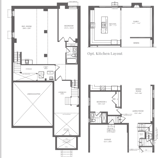
Opt. Finished Basement - Elevation A
