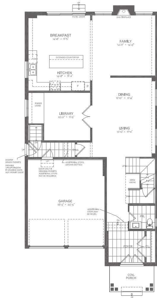
Ground Floor - Elevation A
