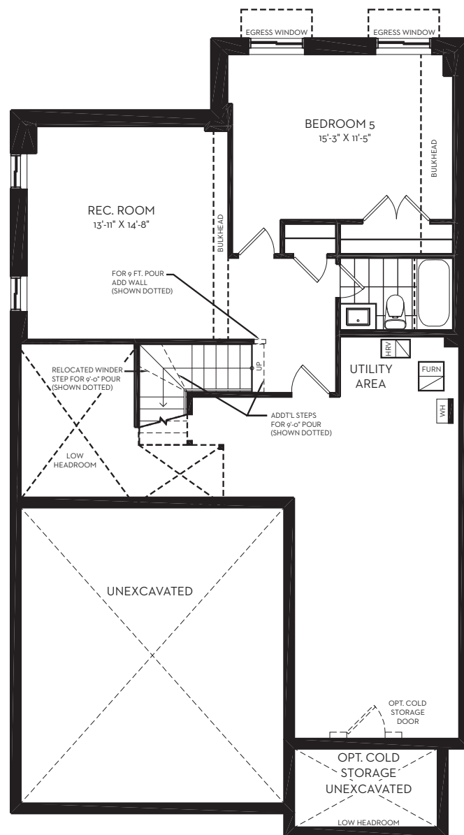
BASEMENT PLAN
