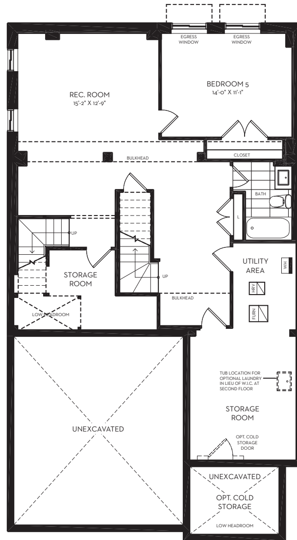
BASEMENT PLAN
