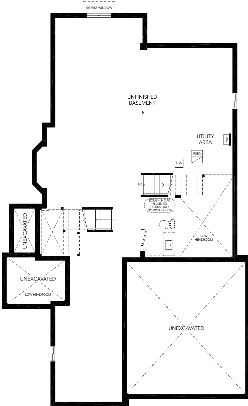
BASEMENT PLAN
