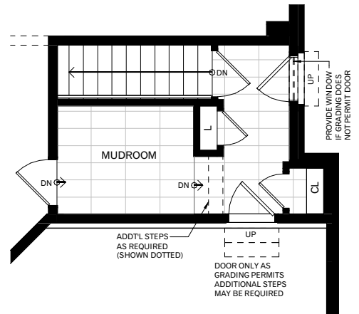
Partial Ground Floor Plan With Opt. Mudroom In Lieu Of Laundry
