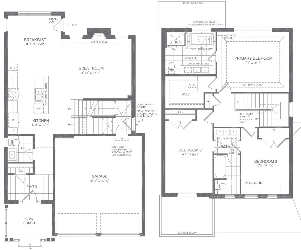
Ground Floor - Elevation A
