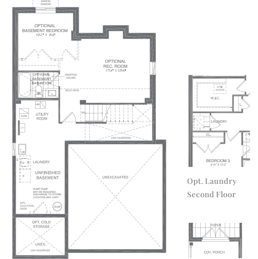
Opt. Finished Basement - Elevation A
