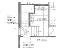
Opt. Mudroom Ground Floor
